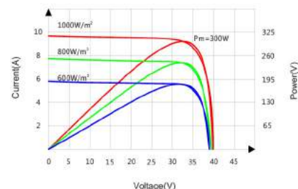
Current-Voltage&Power-Voltage Curve(300W)
