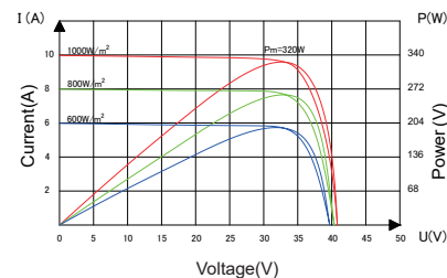
Current-Voltage&Power-Voltage Curve(320W)
