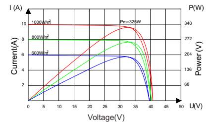
Current-Voltage&Power-Voltage Curve(325W)
