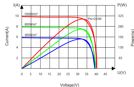
Current-Voltage&Power-Voltage Curve(310W)
